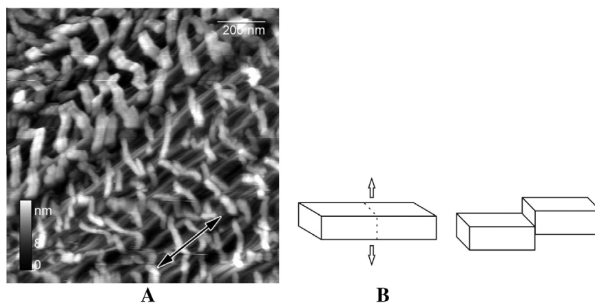
Fig. 7. (A) AFM image of HDPE stretched by 200% in water–ethanol solution. The direction of the stretching coincides with the extrusion axis and is denoted by the arrow. (B) Scheme of disruption of lamellae into fragments.
