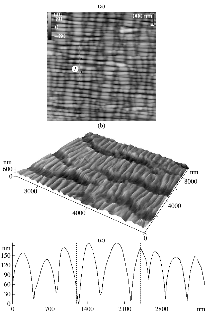
Fig. 2. (a) Atomic-force photomicrograph of a poly(ethylene terephthalate) sample treated with plasma for 1 min and then stretched by 50% at 90°C, (b) its three-dimensional reconstruction, and (c) the profilogram of region I in panel (a).
