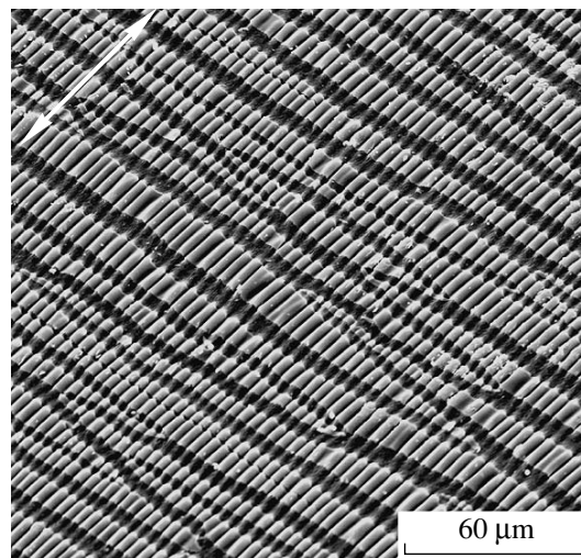
Fig. 1. Scanning electron photomicrograph of a poly(vinyl chloride) sample with a thin (21 nm) platinum coating after stretching the sample by 50% at a rate of 1 mm/min at 90°C. The arrow shows the stretching direction.
